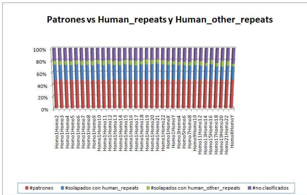
Figura 12: Patrones vs. human_repeats y human_other_repeats (solapamiento \geq 20 )
