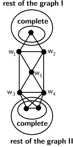
Fig. 13. Structure of G when H has no K_4 .
