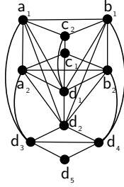
Fig. 6. Graph H_4 , for n = 2 .
