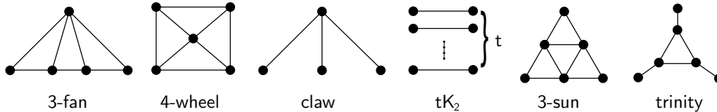
Fig. 8. Some graphs mentioned in the paper.
