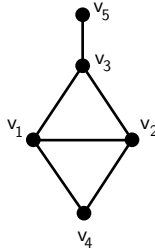
Fig. 12. Subgraph of H when H contains no K_4 and G contains a 1-pyramid.
