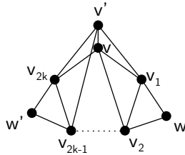
Fig. 1. The graph S_k .
