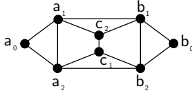
Fig. 7. Graph H_5 , for n = 2 .
