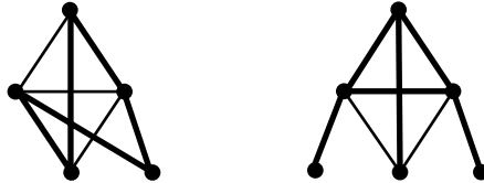
Fig. 10. How the remaining vertices of H can be attached to the K_4 .
