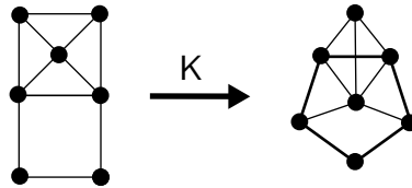
Fig. 9. A clique-perfect graph that is not K-perfect.
