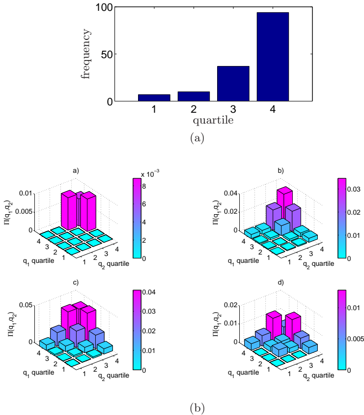
Figure 4: (a) Histogram of Q_y(v) . (b) Probabilities \Pi_y(q_1, q_2) for y = \{1975, 1990, 1996, 2005\} .
