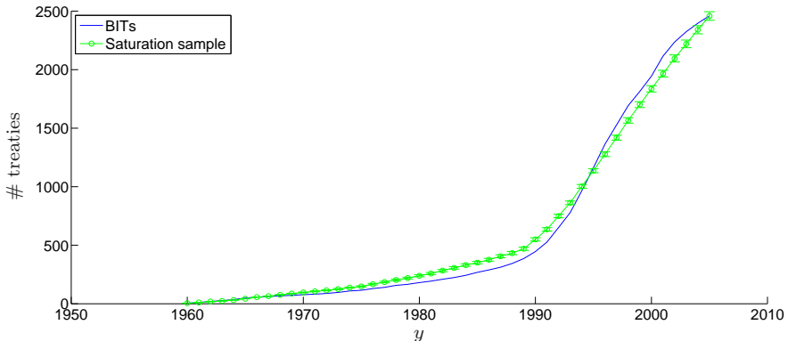
Figure 7: Comparison of the number of treaties signed in the BIT network, to the number of treaties signed by the modified Model B, using \Delta T_y = 0.038|N_y|(|N_y| - 1)/2
