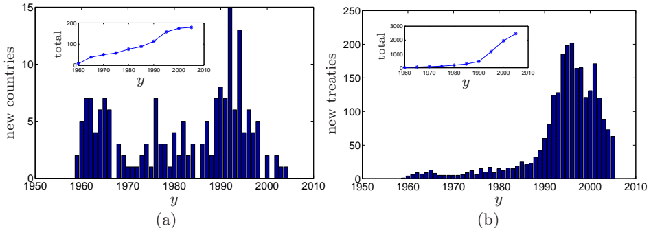
Figure 1: (a) New countries per year. (b) New treaties per year. Note: The insets show cumulative numbers.
