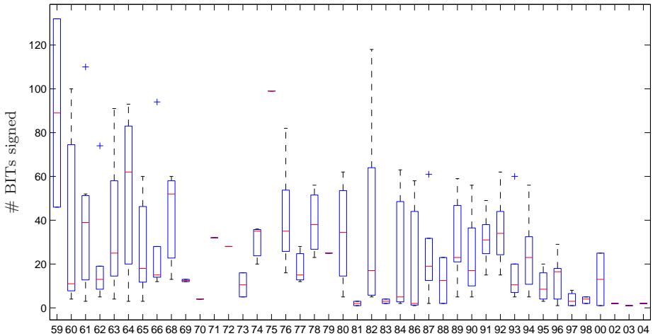
Figure 5: Boxplot of the number of BITs signed by 2005 grouped by the year when countries joined the network.
