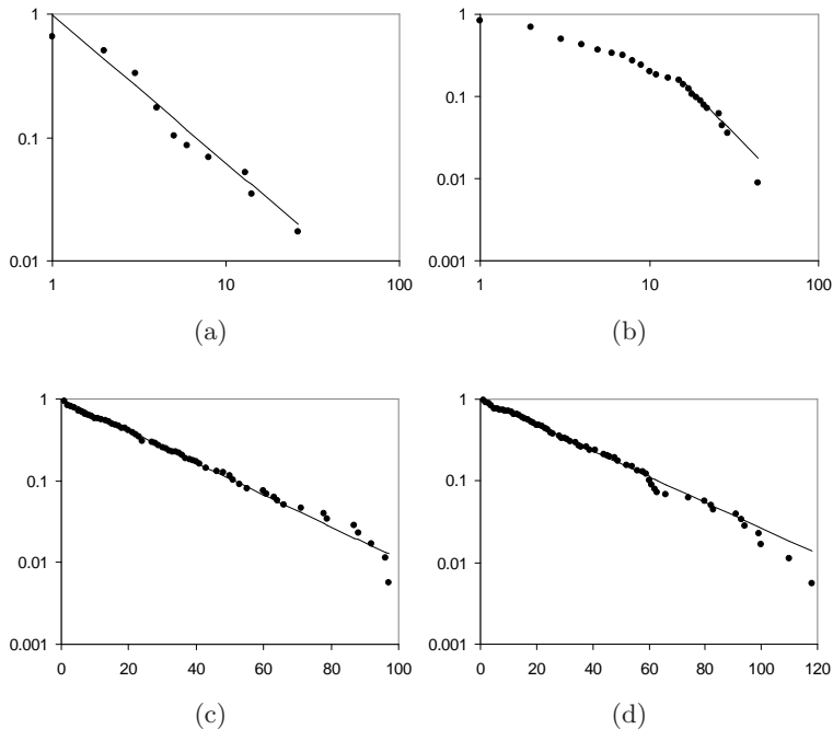
Figure 3: Complementary cumulative distribution function of degrees for years (a) 1975, (b) 1990, (c) 2000, and (d) 2005. Note: (a) and (b) are compared to a power law distribution on a log-log scale, and (c) and (d) are compared to an exponential distribution on a log-linear scale.
