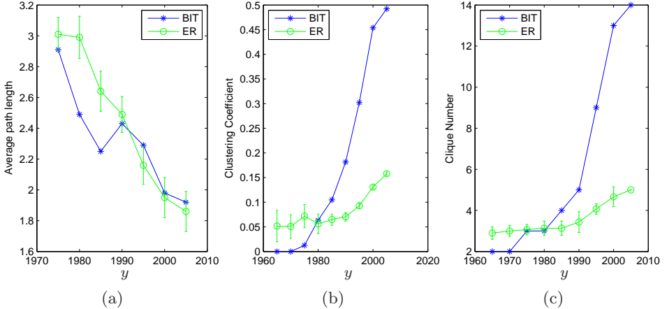
Figure 2: Comparison of the BIT network and ER graphs as a function of time. (a) Average path length. (b) Clustering coefficient. (c) Clique number. Note: The error bars correspond to 1 standard deviation above and below the curve.
