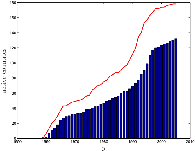
Figure 6: Degree of Germany (bars) compared vs. number of active countries |\mathcal{N}_y| (line) for y \in \{1959, \dots, 2005\} .
