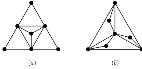
Figure 1: Two graphs G, G' such that K_{1,2}(G) = K_{1,2}(G') . The rightmost one is hereditary clique-Helly, the leftmost one is not even clique-Helly. The leftmost one is UV , the rightmost is not.
