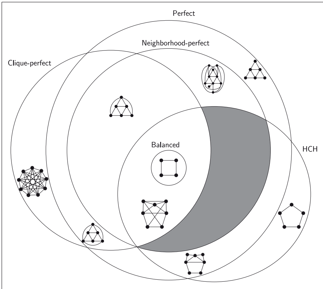
Figure 5: Inclusions and intersections of the studied classes related to neighborhood-perfect graphs, with separating examples. The shaded region corresponds to an empty set.
