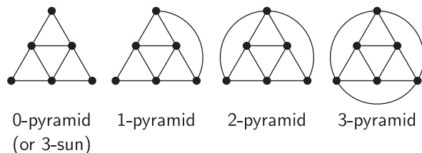
Figure 3: From left to right: 0-, 1-, 2- and 3-pyramid
