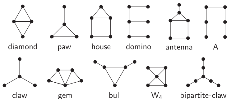
Figure 1: Some small graphs
