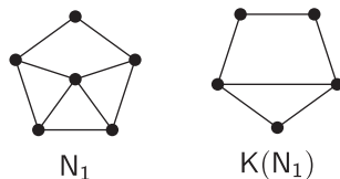
Figure 2: The graph N_1 and its clique graph
