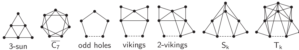
Figure 11: Minimal forbidden induced subgraphs for clique-perfect graphs inside the class of Helly circular-arc graphs. Dashed lines represent induced paths of length 2k - 3 for each k \geq 2 .
