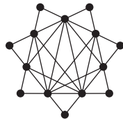
Figure 7: A chordal coordinated odd sun.
