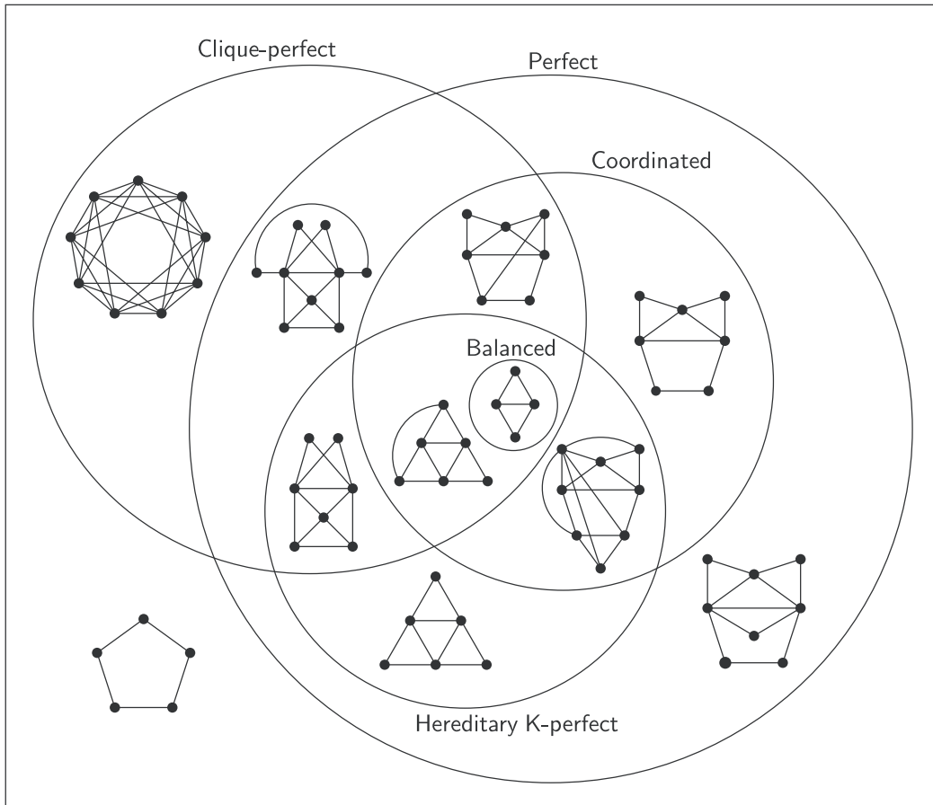
Figure 4: Inclusions and intersections of the studied classes related to coordinated graphs, together with separating examples
