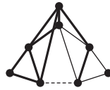
S_k (with a partial viking in bold)
